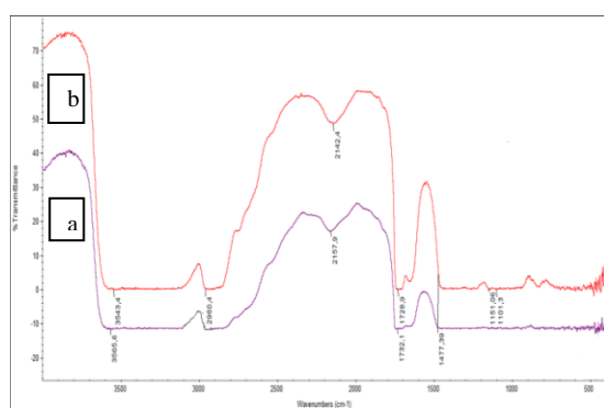
Figure 1. Spectre FTIR des membranes PVA/GA et PVA/GA/ \beta CD
